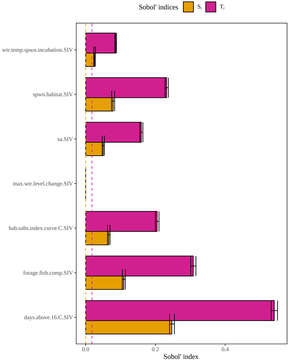
Figure 7. Results of a sensitivity analysis for the whitebassLacCurveCSubsIndex model based on a multiplicative mean structure. Dashed lines represent baseline numerical approximation error for S_i and T_i ( i.e. , dummy variables).
