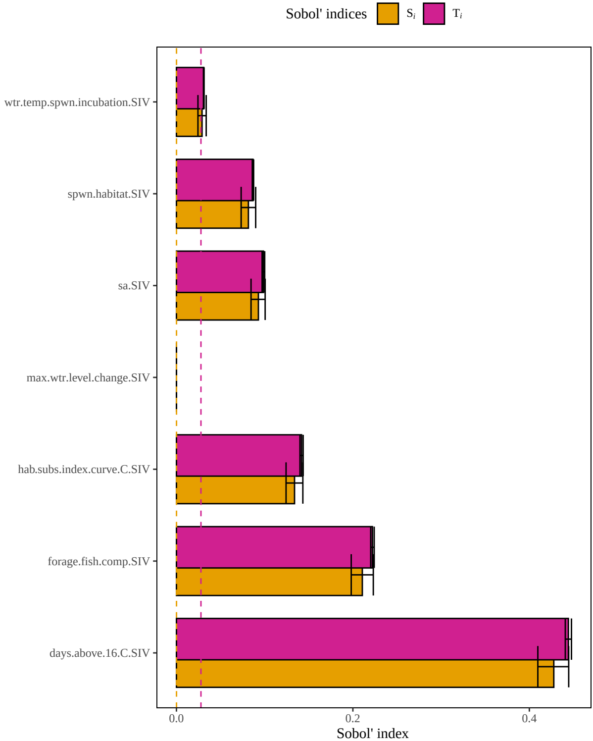
Figure 5. Results of a sensitivity analysis for the whitebassLacCurveCSubsIndex model based on a geometric mean structure. Dashed lines represent baseline numerical approximation error for S_i and T_i ( i.e. , dummy variables).
